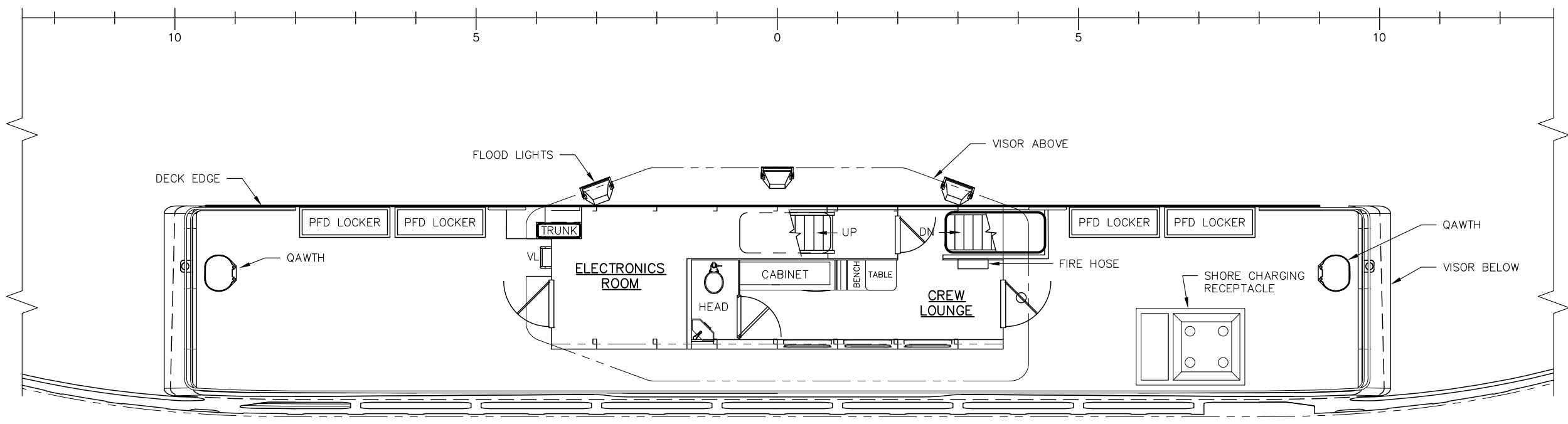
PLAN 5-4A UPPER DECK, CREW ONLY 1/8"=1'-0"
