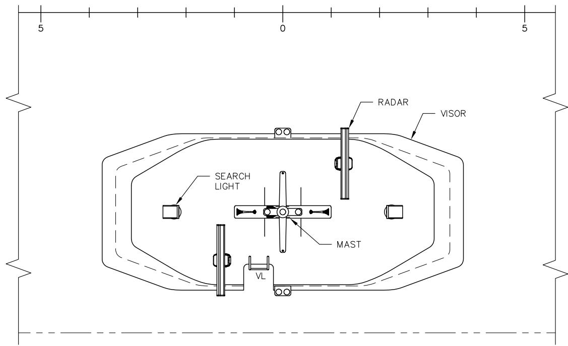
PLAN 5-3C PILOTHOUSE TOP, CREW ONLY 1/8"=1'-0"
