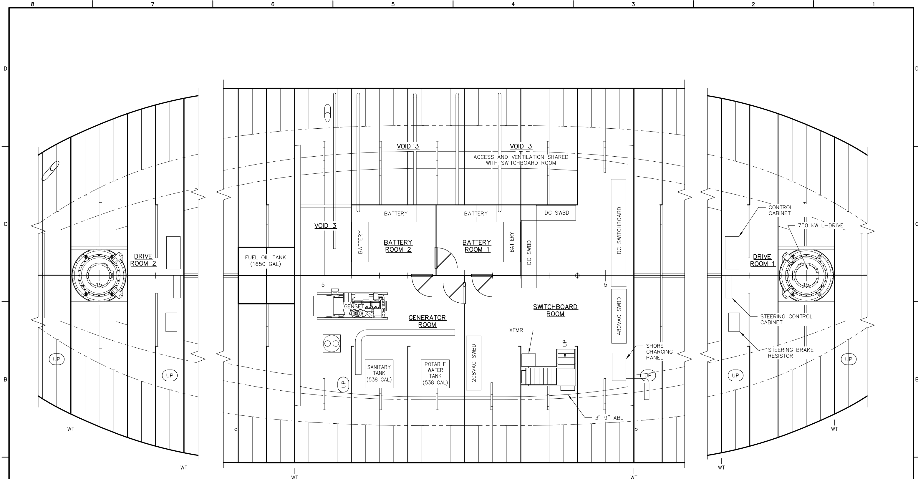
PLAN 6-5C MACHINERY ARRANGEMENT 1/8"=1'-0"
