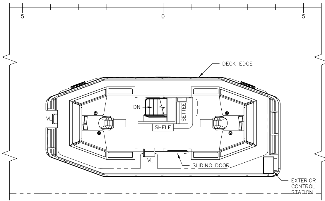
PLAN 5-6C PILOTHOUSE DECK, CREW ONLY 1/8"=1'-0"
