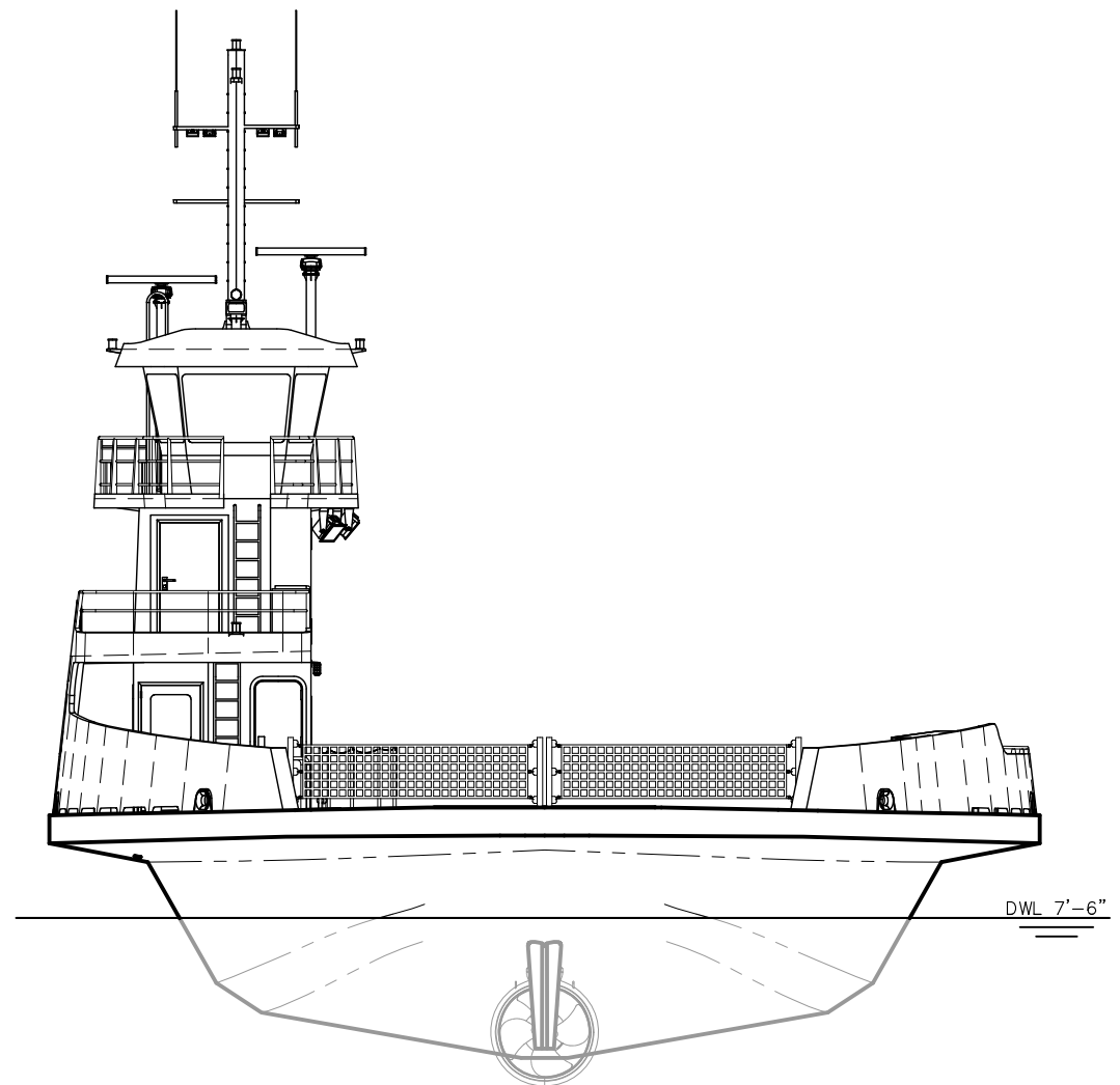
END VIEW 2-6B NO. 1 END (ANACORTES) 3/32"=1'-0"
