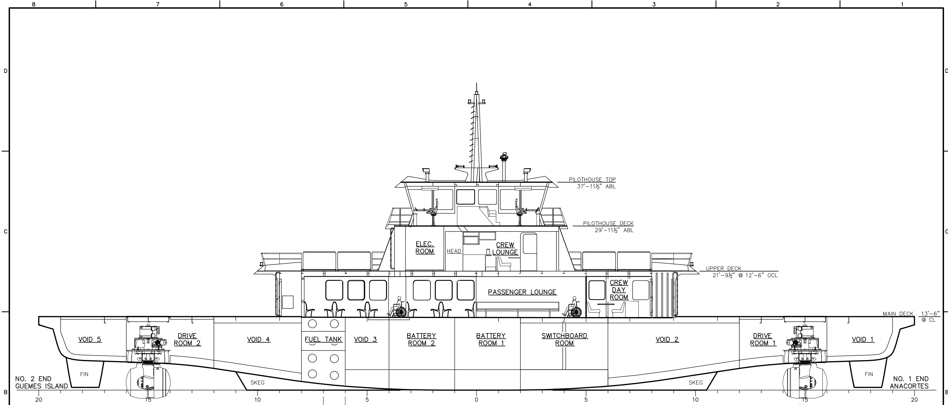
INBOARD PROFILE 3-4B HULL ON CENTERLINE HOUSE ON 16'-6" OCL 3/32"=1'-0"
