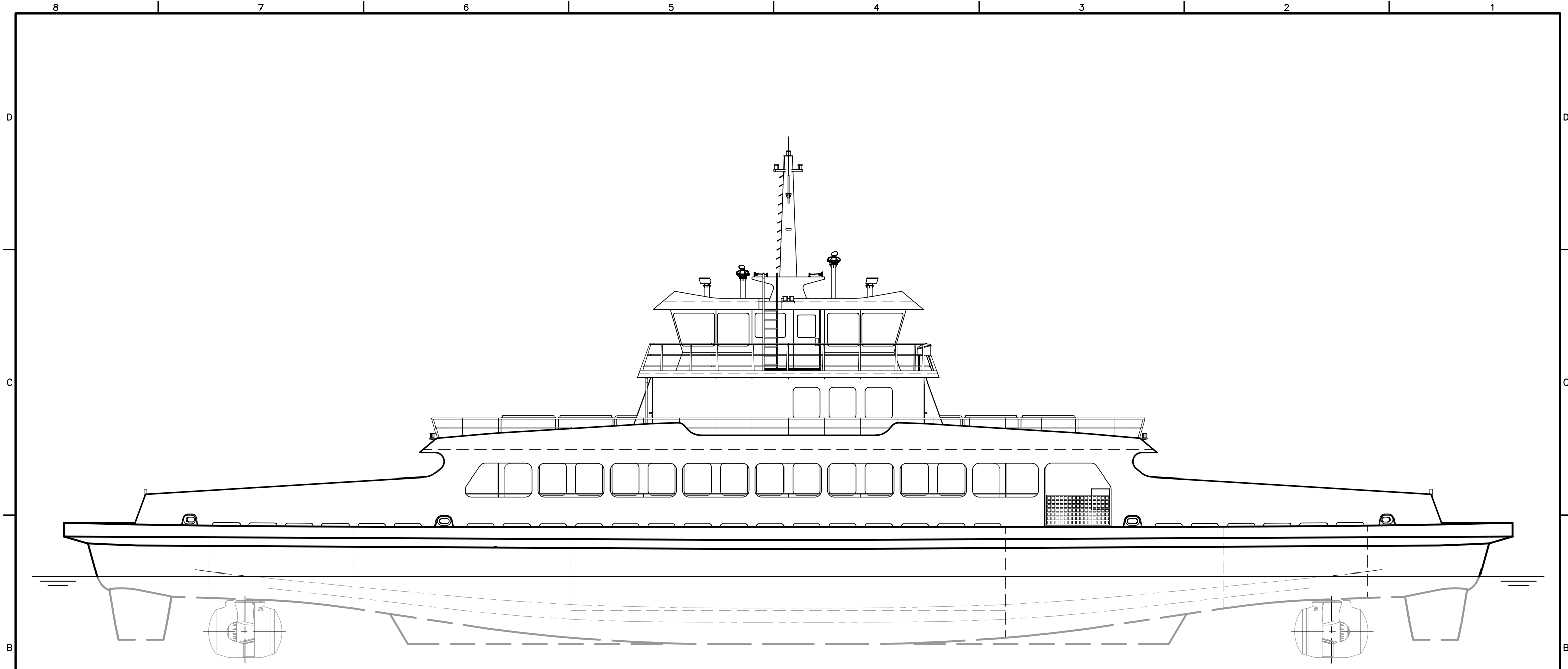
PROFILE 1-5B OUTBOARD PROFILE 3/32"=1'-0"
